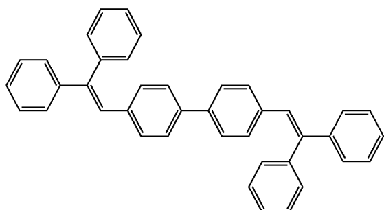
[Chemical Formula 5]
