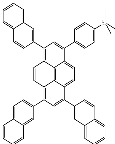
[Chemical Formula 9]
