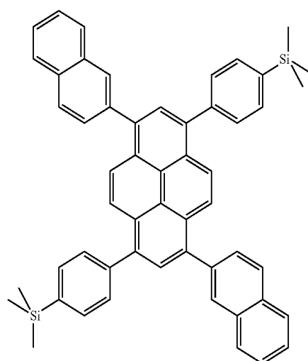
[Chemical Formula 7]
