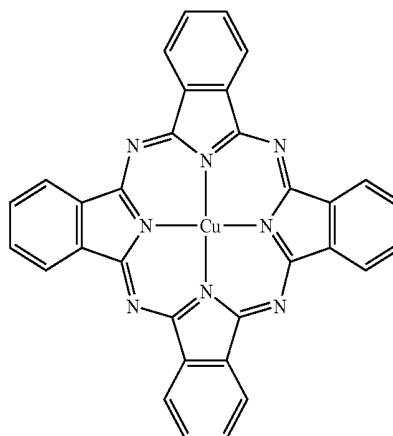
[Chemical Formula 2]
