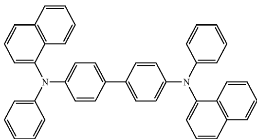
[Chemical Formula 3]
